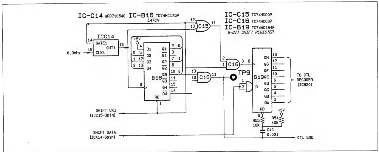
Fig. 4-3-18. CTL Blank Detection Circuit (CD-35 Board)
